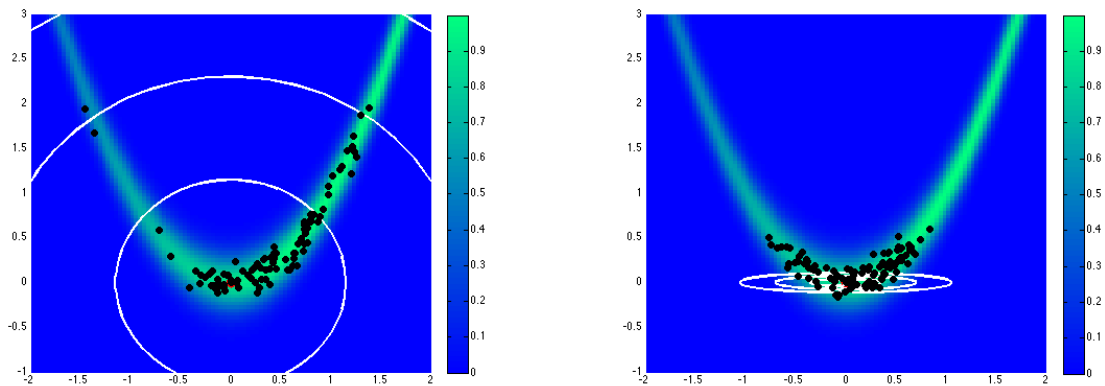
(a) Proposal covariance defined from uniform prior.
