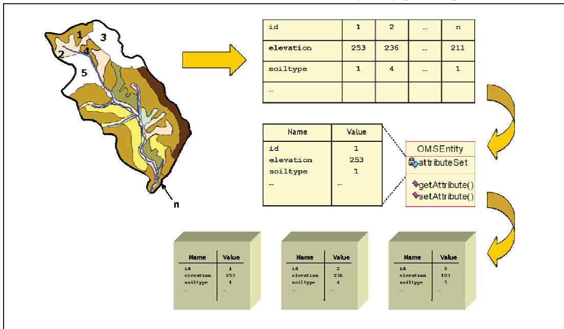
Figure 3. Representing spatial model entities as OMSEntity objects
