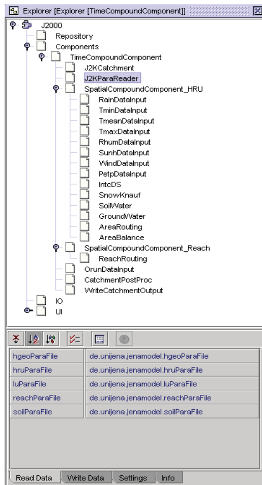
Figure 4. Composition of J2000 components with the model builder
